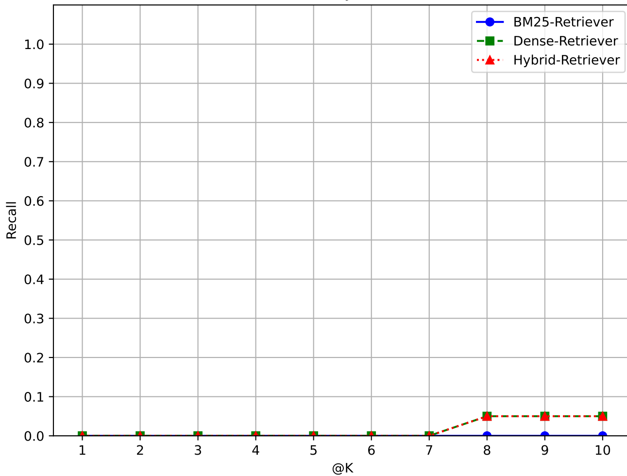
Query 45
